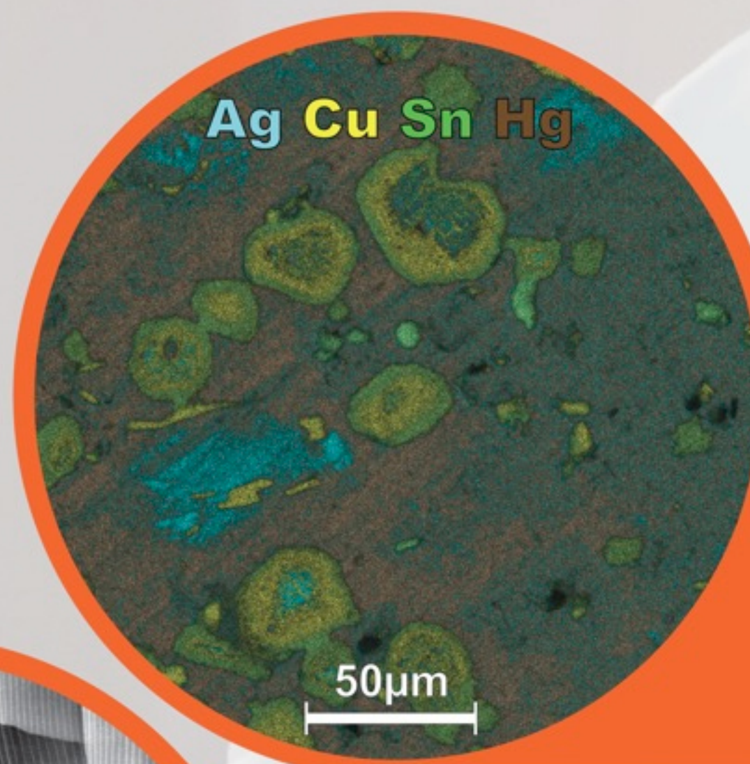
EDXS elemental map of dental amalgam.
